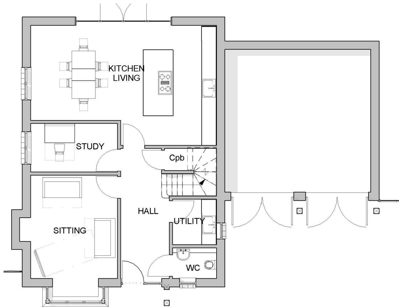
Plot 2 - Ground Floor Plan as Proposed 1 : 100
