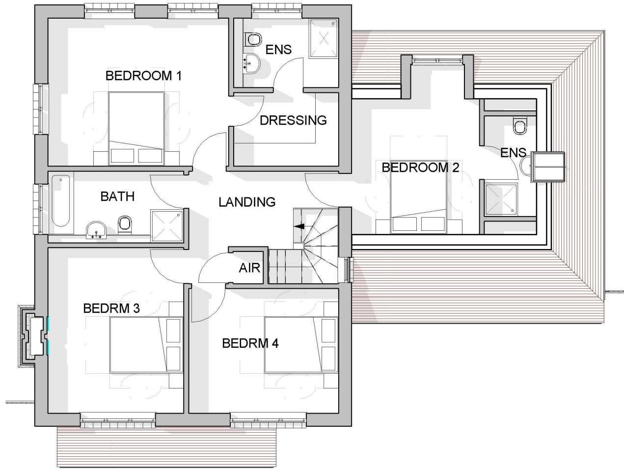
Plot 2 - First Floor Plan as Proposed 1 : 100
